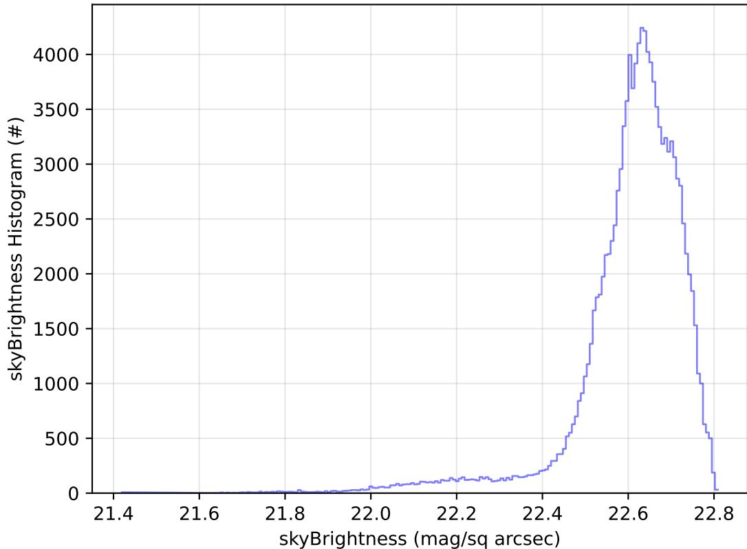
ddf_acor_sf15_lsf40_lsr20_v3.4_10yrs WFD u band: skyBrightness Histogram
