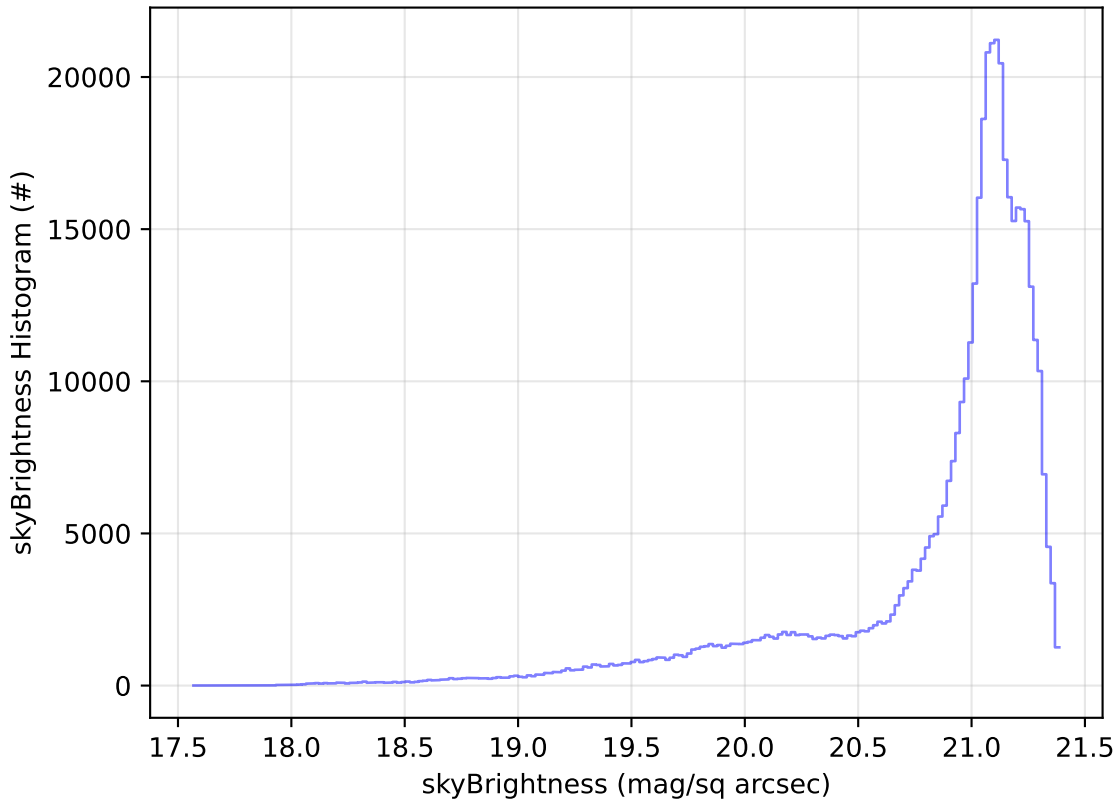
ddf_acor_sf15_lsf40_lsr20_v3.4_10yrs WFD r band: skyBrightness Histogram
