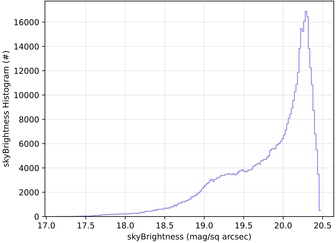
ddf_acor_sf15_lsf40_lsr20_v3.4_10yrs WFD i band: skyBrightness Histogram
