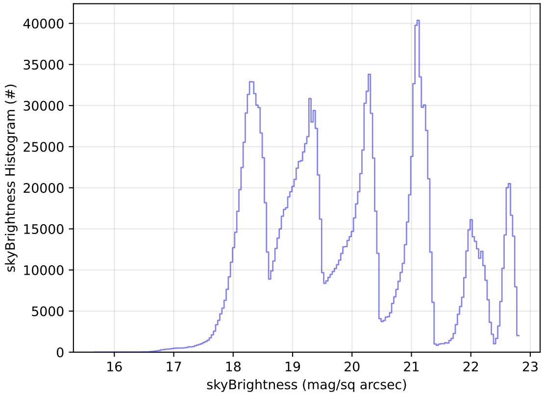
ddf_acor_sf15_ls40_lsr20_v3.4_10yrs WFD all bands: skyBrightness Histogram
