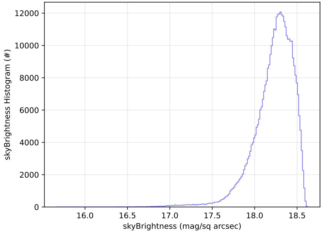
ddf_acor_sf15_lsf40_lsr20_v3.4_10yrs All sky y band: skyBrightness Histogram
