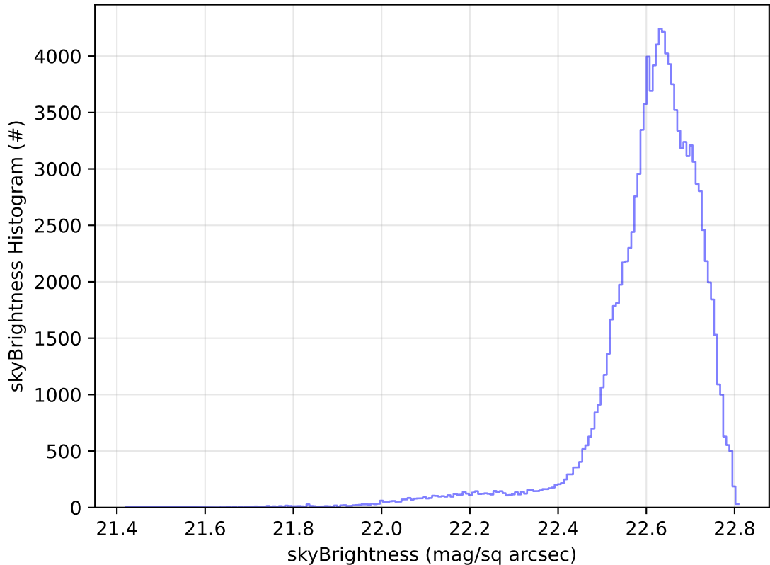
ddf_acor_sf15_lsf40_lsr20_v3.4_10yrs All sky u band: skyBrightness Histogram
