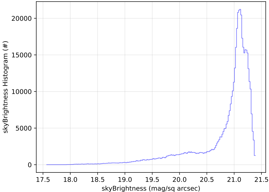
ddf_acor_sf15_lsf40_lsr20_v3.4_10yrs All sky r band: skyBrightness Histogram
