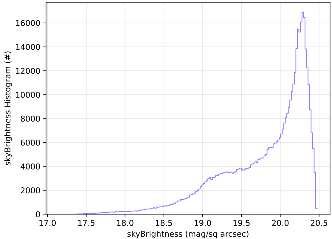
ddf_acor_sf15_lsf40_lsr20_v3.4_10yrs All sky i band: skyBrightness Histogram
