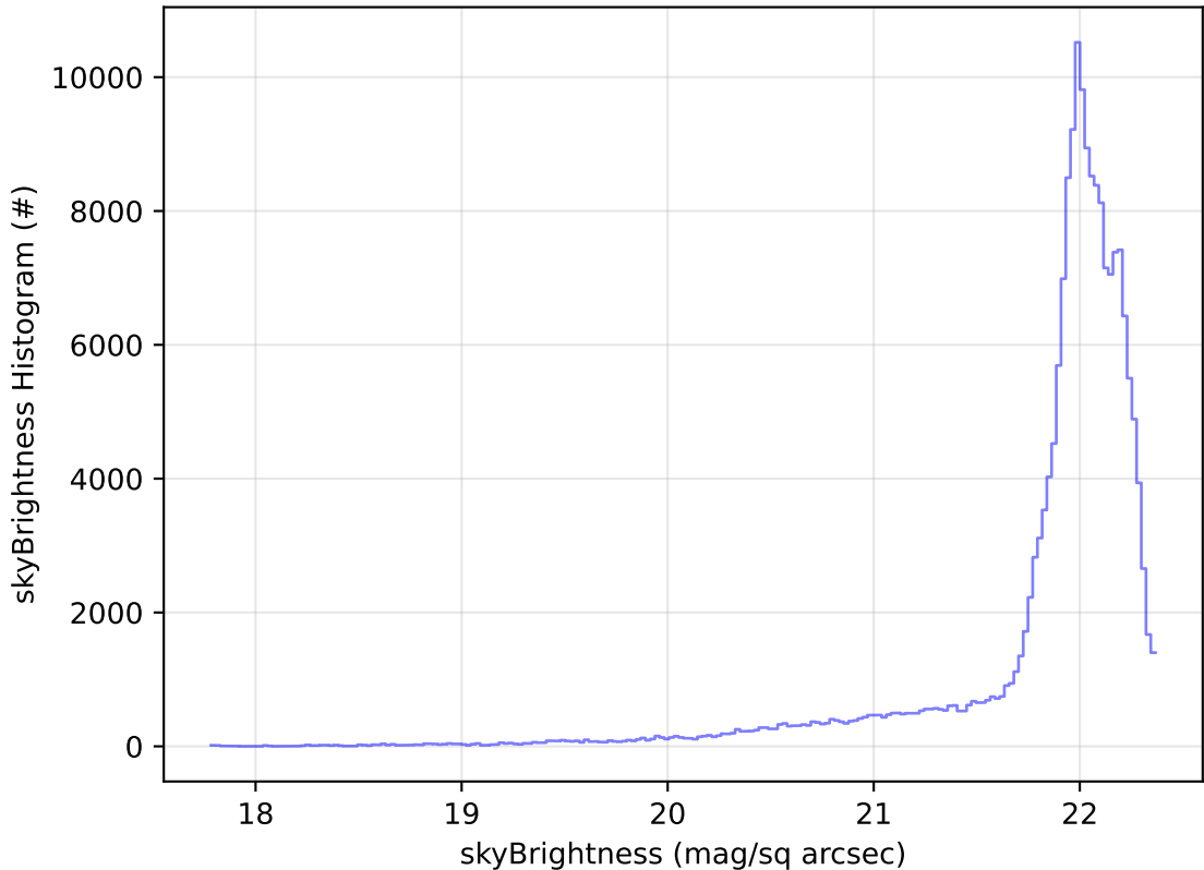
ddf_acor_sf15_ls40_lsr20_v3.4_10yrs All sky g band: skyBrightness Histogram
