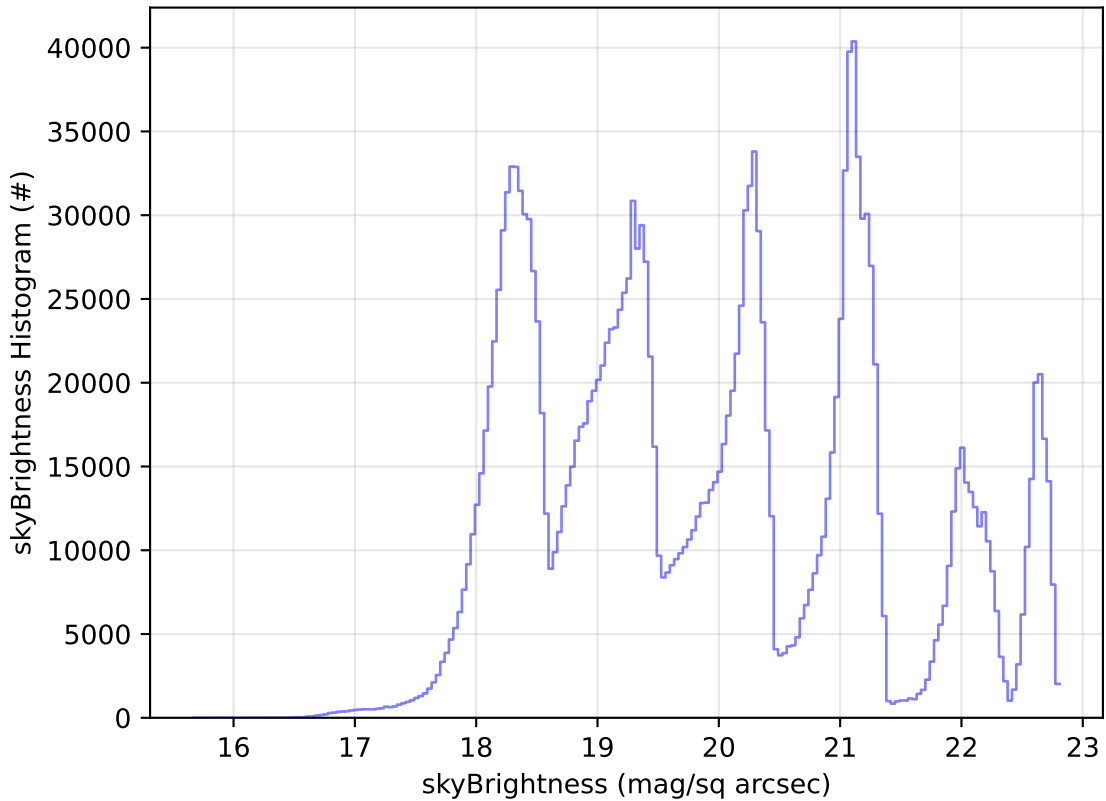
ddf_acor_sf15_lsf40_lsr20_v3.4_10yrs All sky all bands: skyBrightness Histogram
