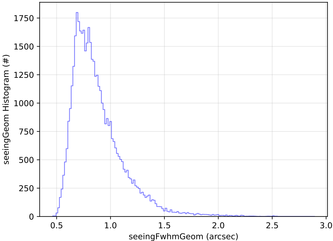
ddf_acor_sf15_lsf40_lsr20_v3.4_10yrs Yr 1 z band: seeingGeom Histogram
