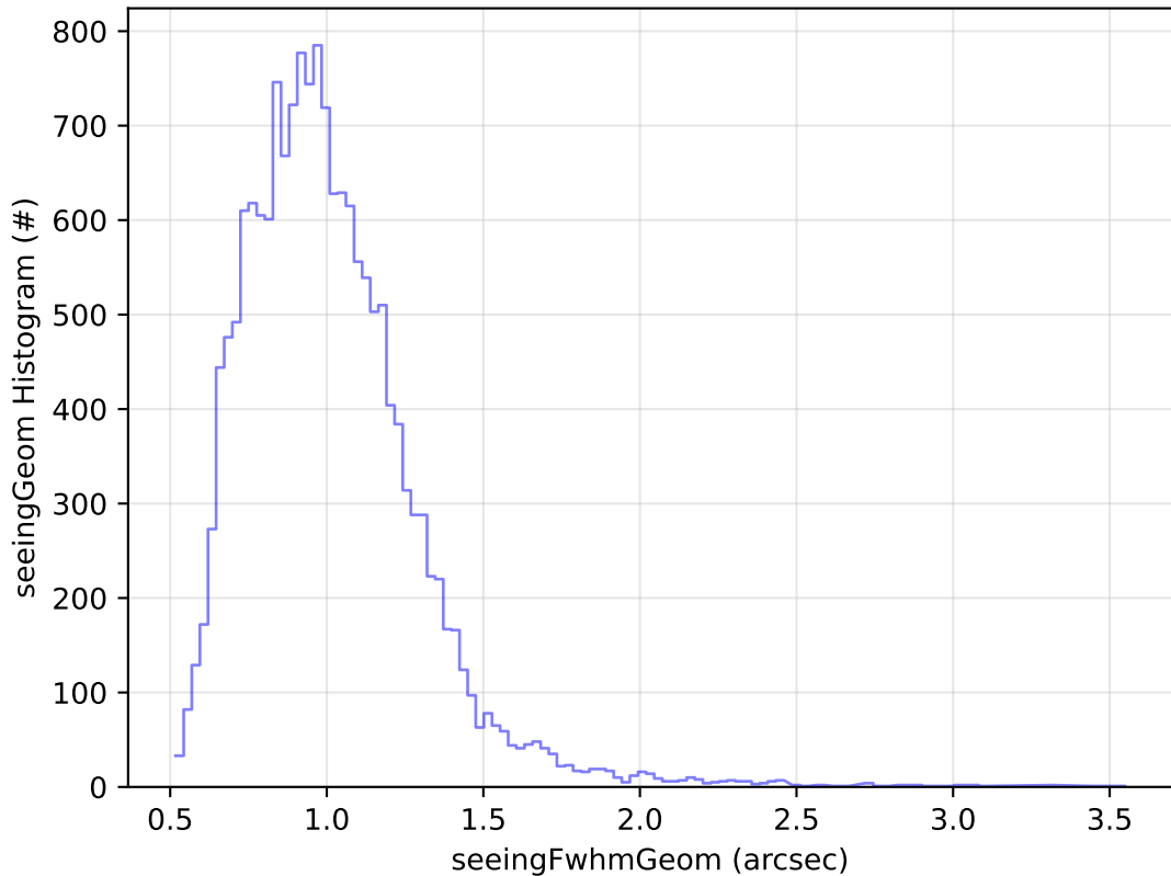
ddf_acor_sf15_lsf40_lsr20_v3.4_10yrs Yr 1 u band: seeingGeom Histogram
