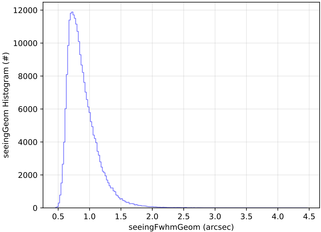
ddf_acor_sf15_lsf40_lsr20_v3.4_10yrs Yr 1 all bands: seeingGeom Histogram
