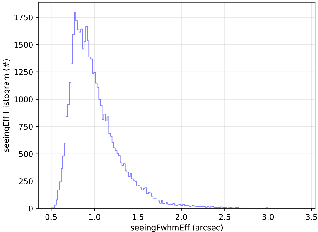
ddf_acor_sf15_lsf40_lsr20_v3.4_10yrs Yr 1 z band: seeingEff Histogram
