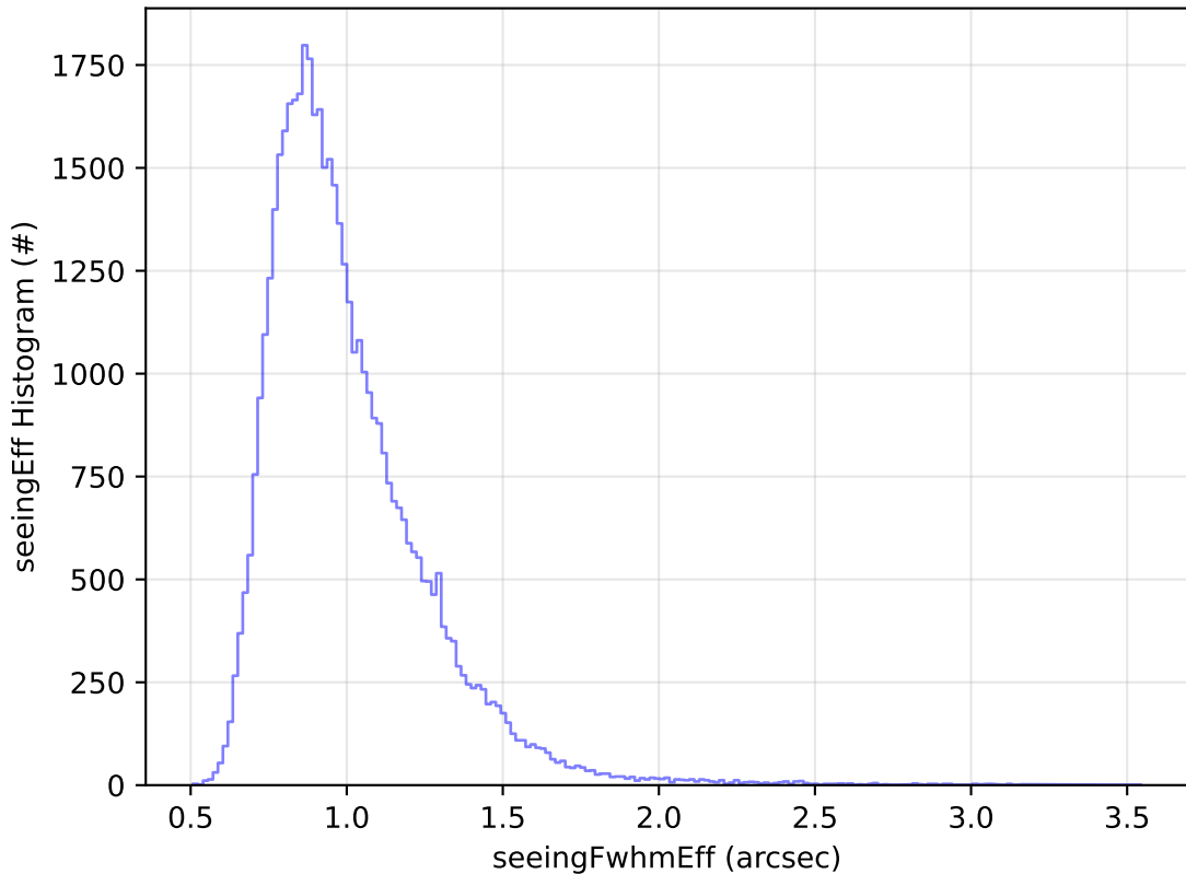
ddf_acor_sf15_lsf40_lsr20_v3.4_10yrs Yr 1 y band: seeingEff Histogram
