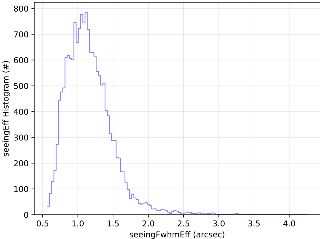
ddf_acor_sf15_lsf40_lsr20_v3.4_10yrs Yr 1 u band: seeingEff Histogram
