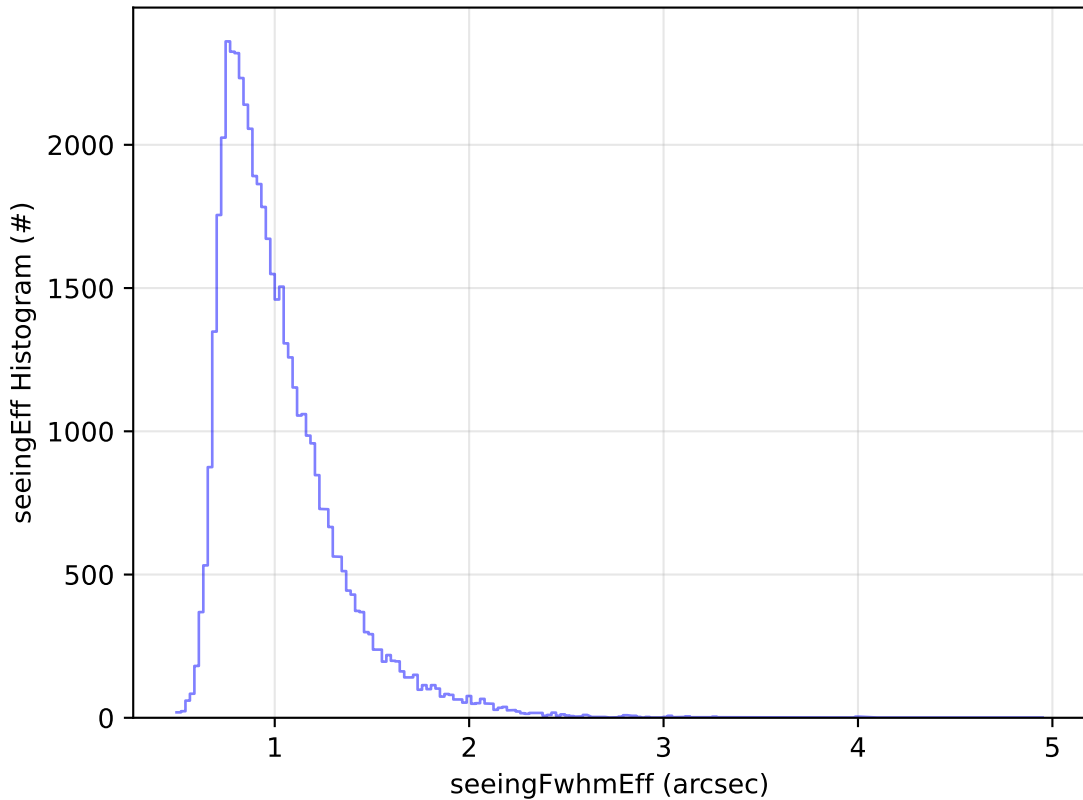
ddf_acor_sf15_lsf40_lsr20_v3.4_10yrs Yr 1 r band: seeingEff Histogram
