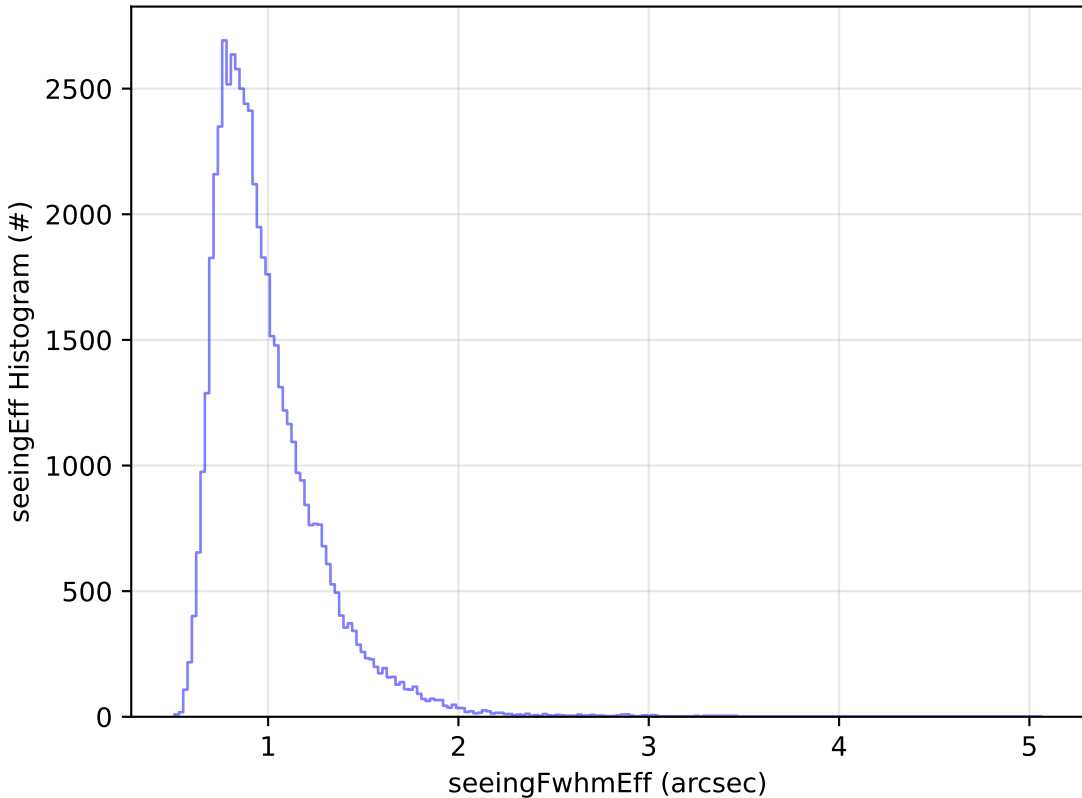
ddf_acor_sf15_lsf40_lsr20_v3.4_10yrs Yr 1 i band: seeingEff Histogram
