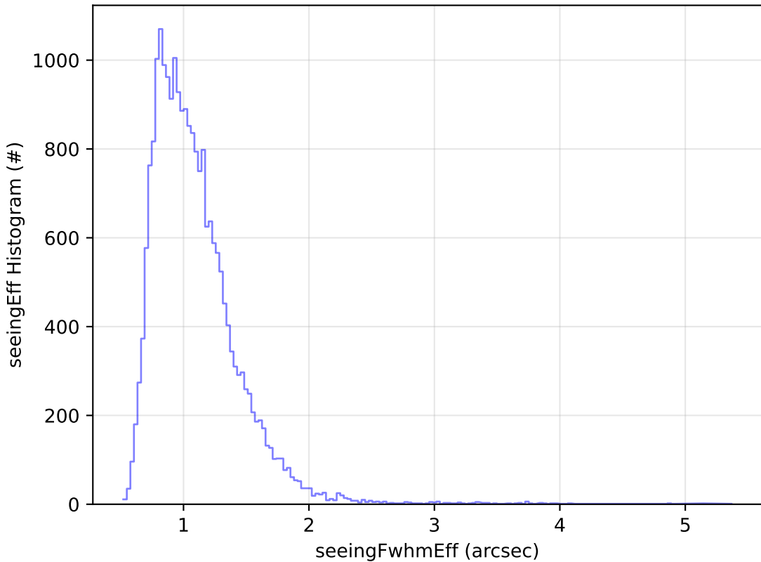
ddf_acor_sf15_lsf40_lsr20_v3.4_10yrs Yr 1 g band: seeingEff Histogram
