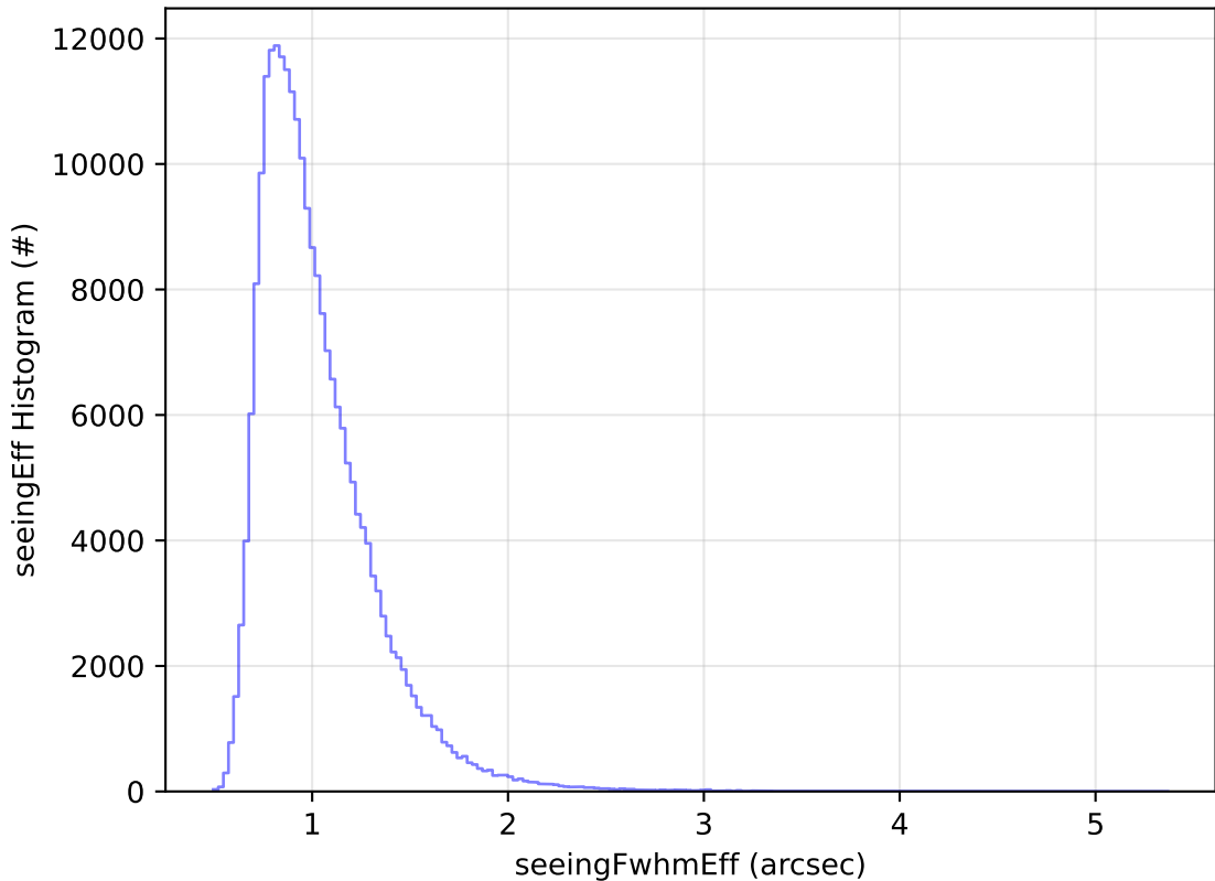
ddf_acor_sf15_Isf40_Isr20_v3.4_10yrs Yr 1 all bands: seeingEff Histogram
