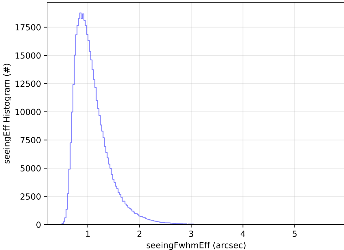
ddf_acor_sf15_lsf40_lsr20_v3.4_10yrs WFD z band: seeingEff Histogram
