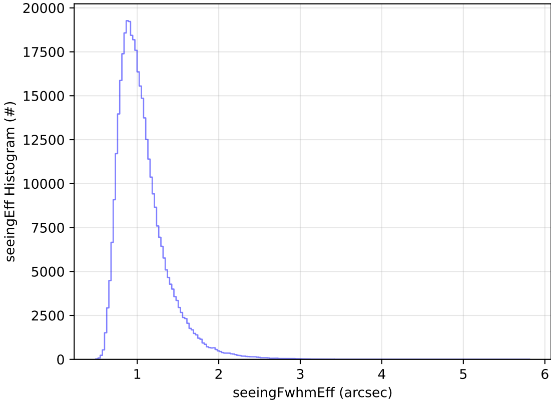
ddf_acor_sf15_lsf40_lsr20_v3.4_10yrs WFD y band: seeingEff Histogram
