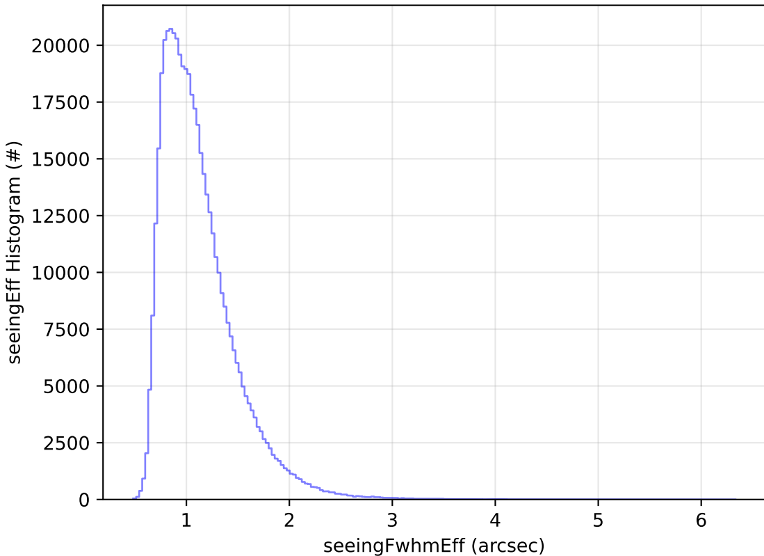
ddf_acor_sf15_lsf40_lsr20_v3.4_10yrs WFD r band: seeingEff Histogram
