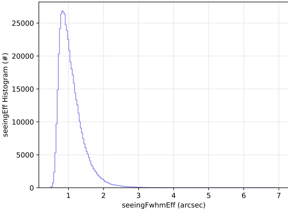
ddf_acor_sf15_lsf40_lsr20_v3.4_10yrs WFD i band: seeingEff Histogram
