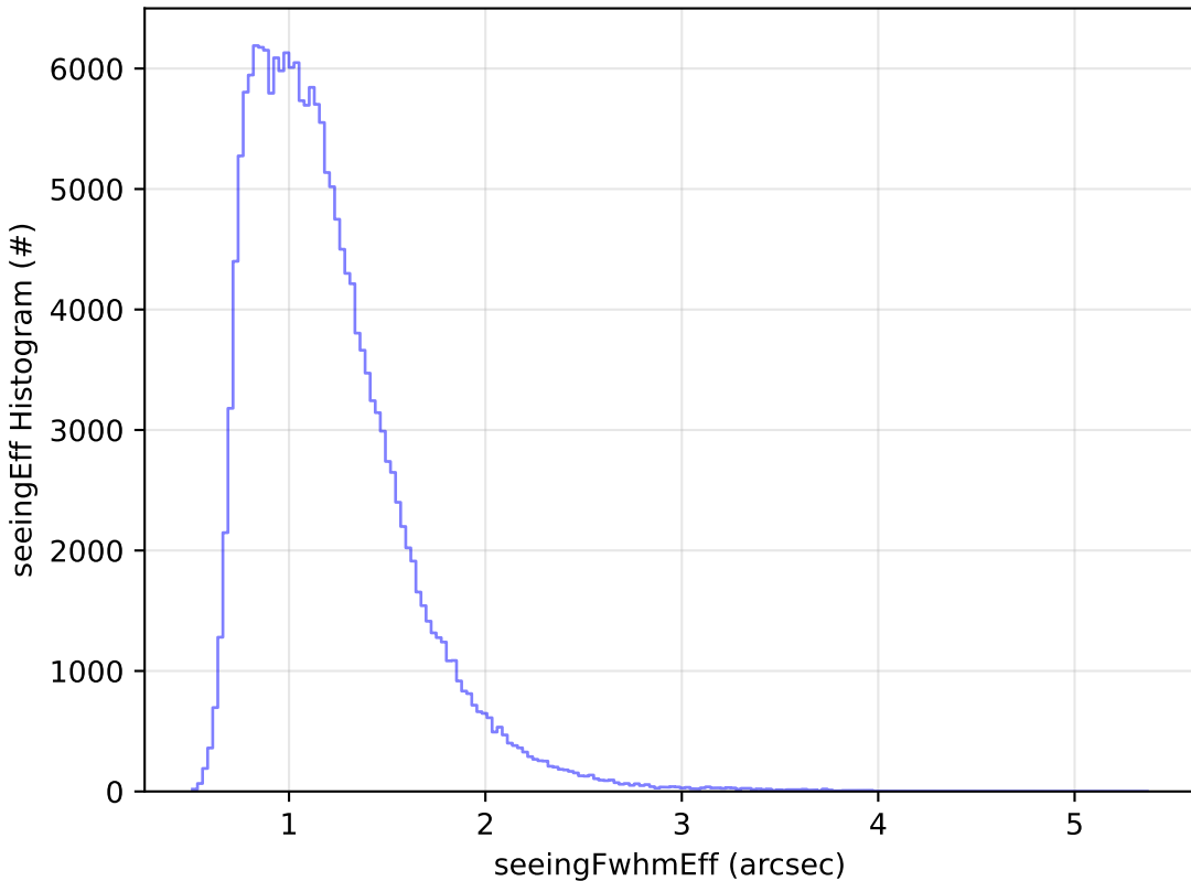
ddf_acor_sf15_lsf40_lsr20_v3.4_10yrs WFD g band: seeingEff Histogram
