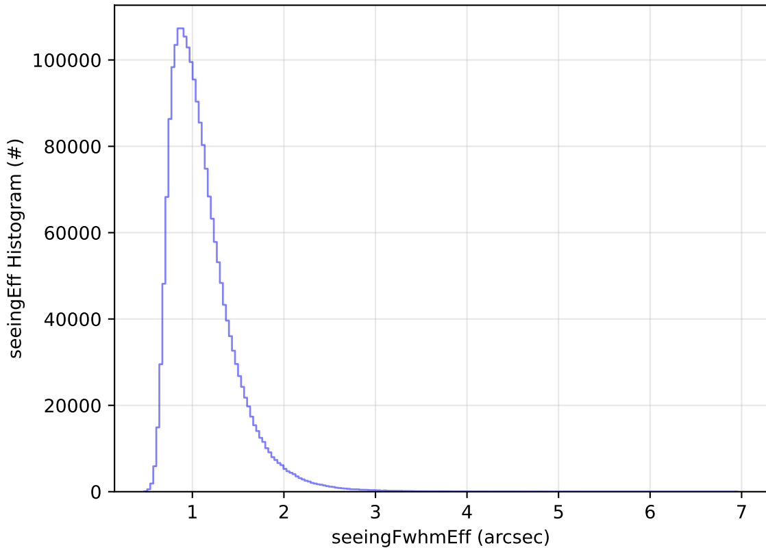
ddf_acor_sf15_lsf40_lsr20_v3.4_10yrs WFD all bands: seeingEff Histogram
