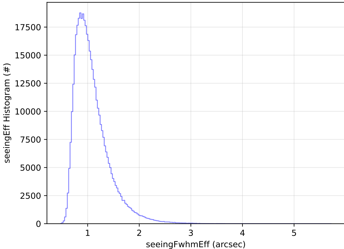
ddf_acor_sf15_lsf40_lsr20_v3.4_10yrs All sky z band: seeingEff Histogram
