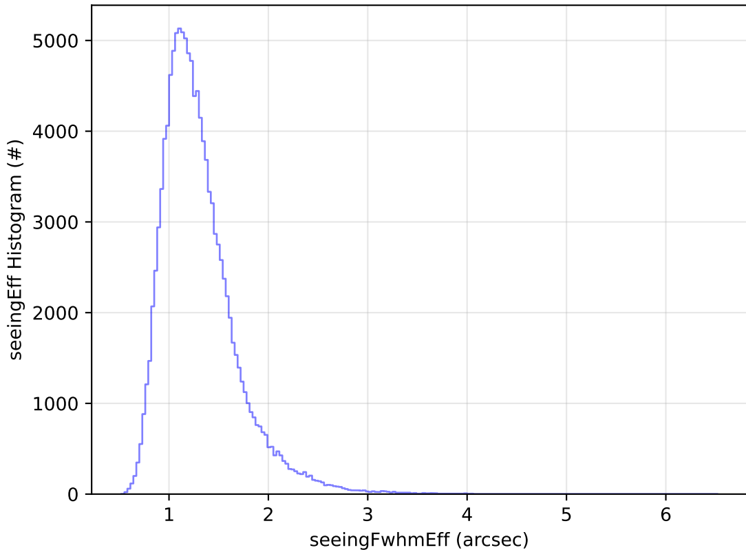
ddf_acor_sf15_ls40_lsr20_v3.4_10yrs All sky u band: seeingEff Histogram
