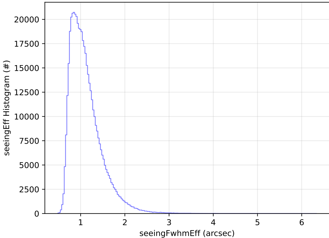
ddf_acor_sf15_lsf40_lsr20_v3.4_10yrs All sky r band: seeingEff Histogram
