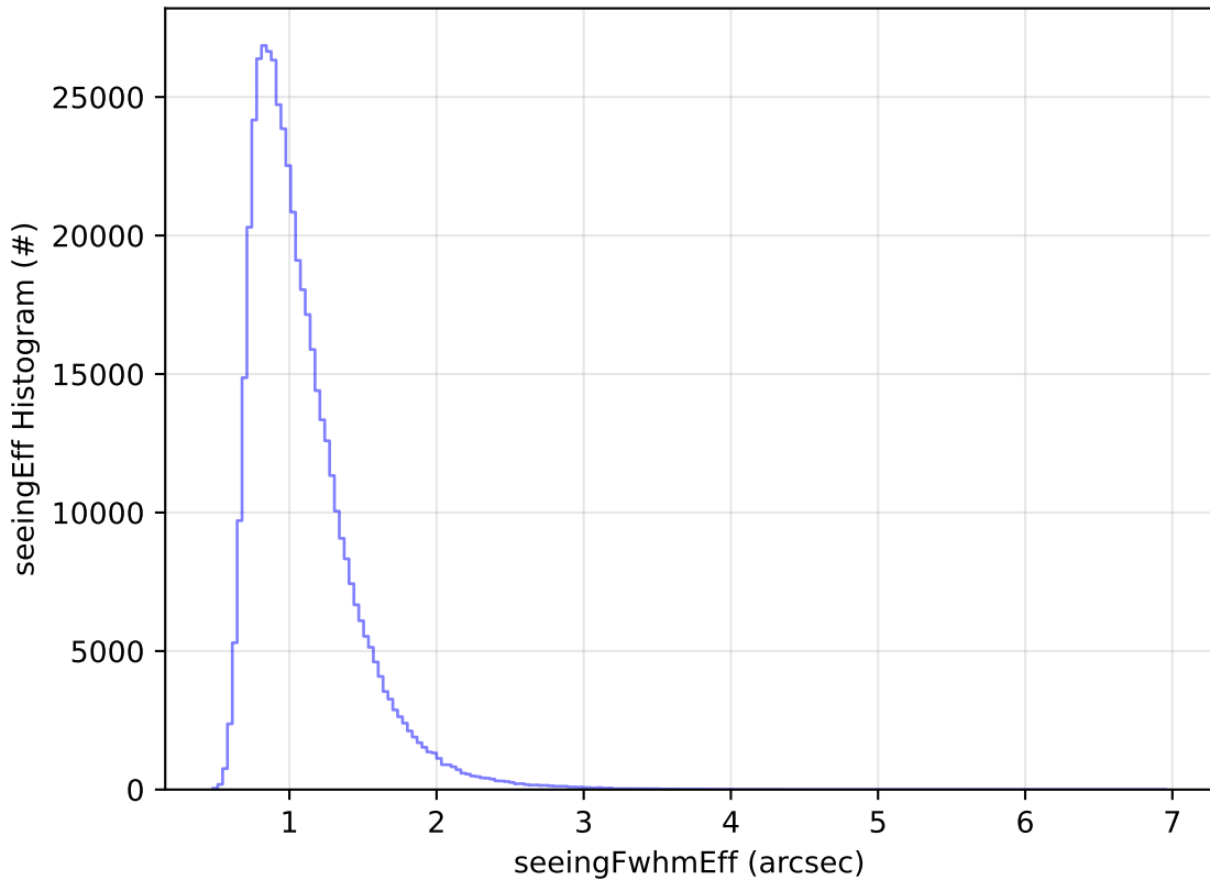
ddf_acor_sf15_lsf40_lsr20_v3.4_10yrs All sky i band: seeingEff Histogram
