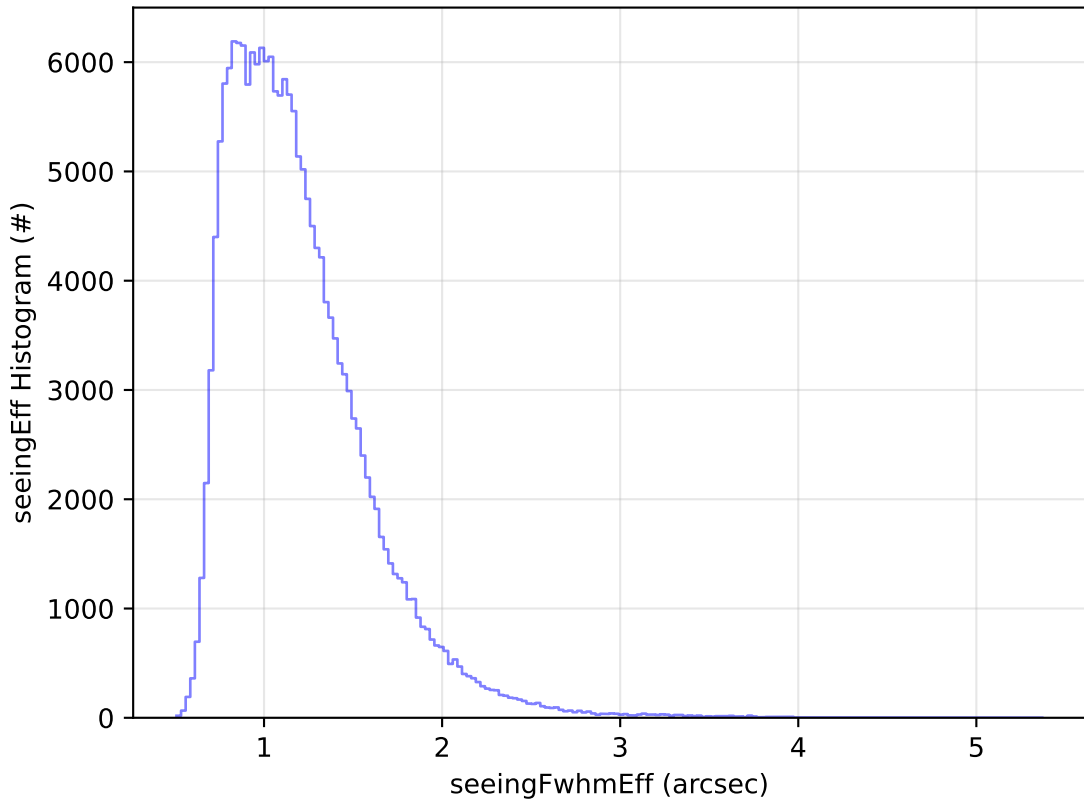
ddf_acor_sf15_ls40_lsr20_v3.4_10yrs All sky g band: seeingEff Histogram
