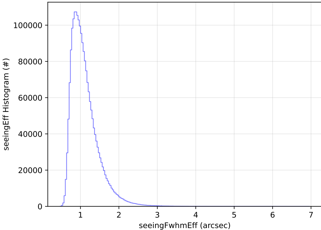
ddf_acor_sf15_lsf40_lsr20_v3.4_10yrs All sky all bands: seeingEff Histogram
