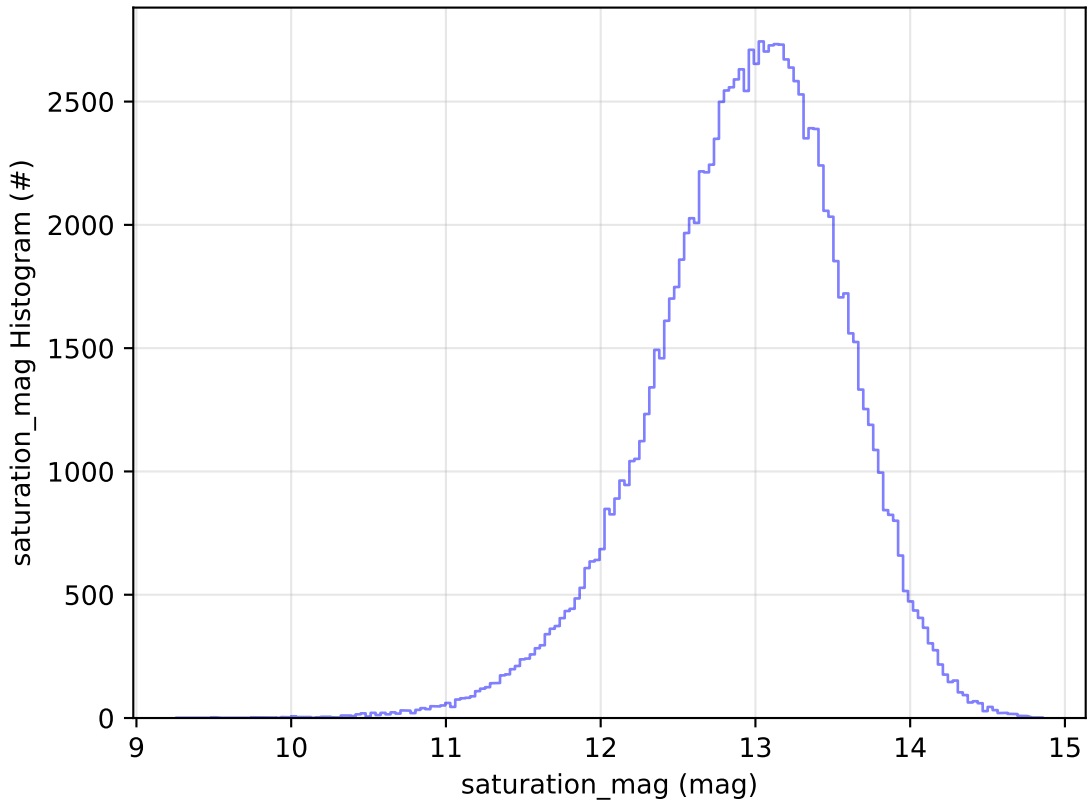
ddf_acor_sf15_lsf40_lsr20_v3.4_10yrs WFD u band: saturation_mag Histogram
