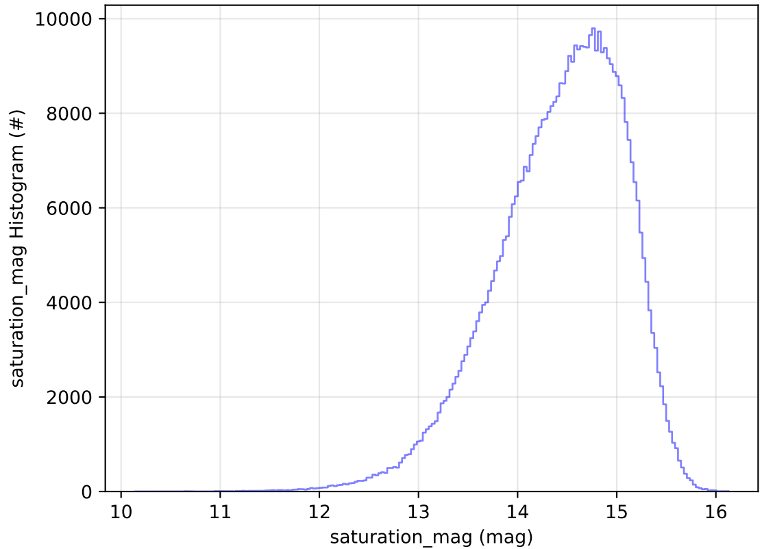
ddf_acor_sf15_lsf40_lsr20_v3.4_10yrs WFD i band: saturation_mag Histogram
