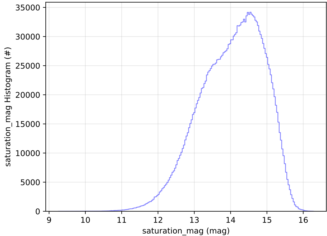
ddf_acor_sf15_lsf40_lsr20_v3.4_10yrs WFD all bands: saturation_mag Histogram
