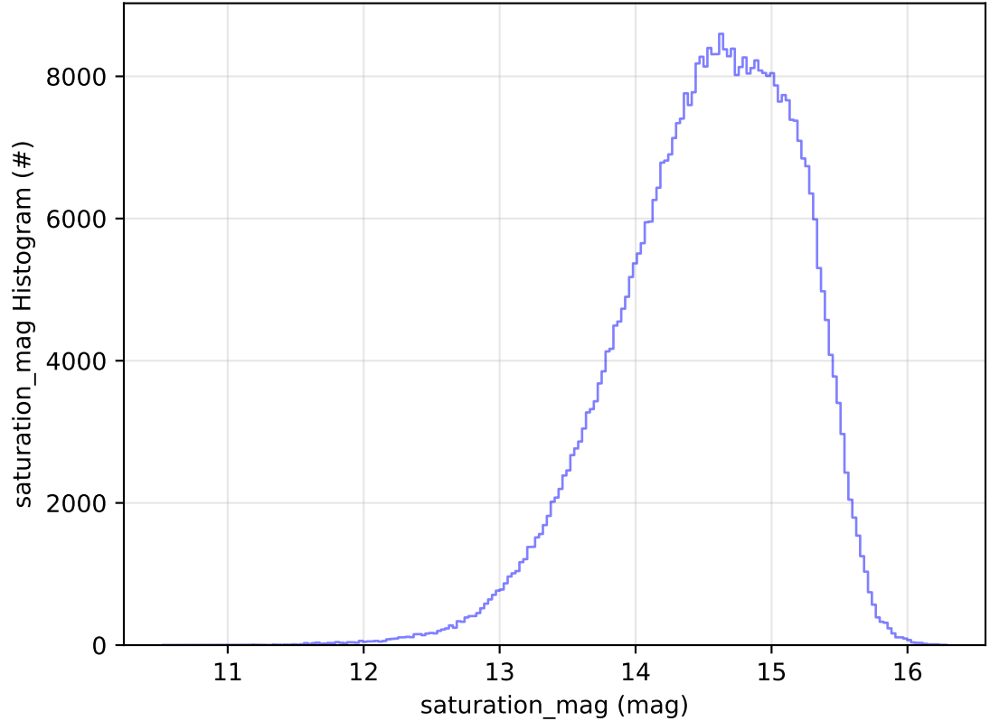
ddf_acor_sf15_lsf40_lsr20_v3.4_10yrs All sky r band: saturation_mag Histogram
