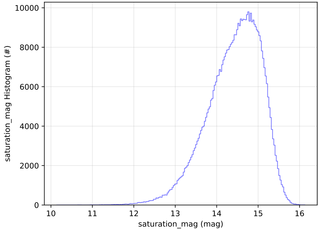
ddf_acor_sf15_lsf40_lsr20_v3.4_10yrs All sky i band: saturation_mag Histogram
