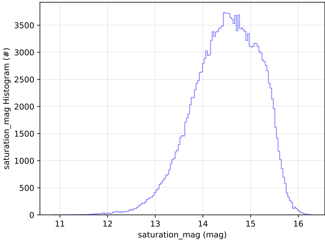
ddf_acor_sf15_lsf40_lsr20_v3.4_10yrs All sky g band: saturation_mag Histogram
