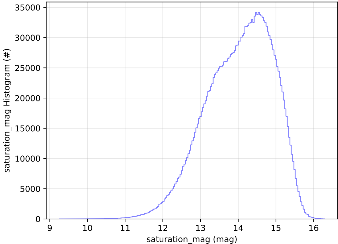
ddf_acor_sf15_lsf40_lsr20_v3.4_10yrs All sky all bands: saturation_mag Histogram
