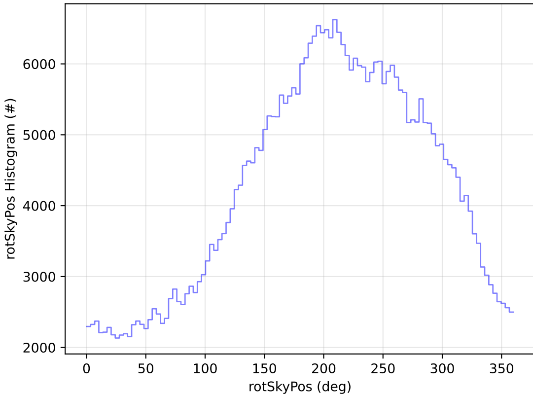
ddf_acor_sf15_lsf40_lsr20_v3.4_10yrs WFD z band: rotSkyPos Histogram
