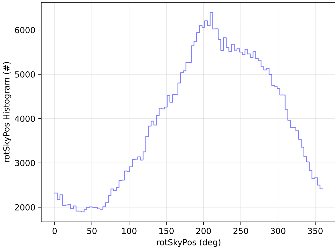
ddf_acor_sf15_lsf40_lsr20_v3.4_10yrs WFD y band: rotSkyPos Histogram
