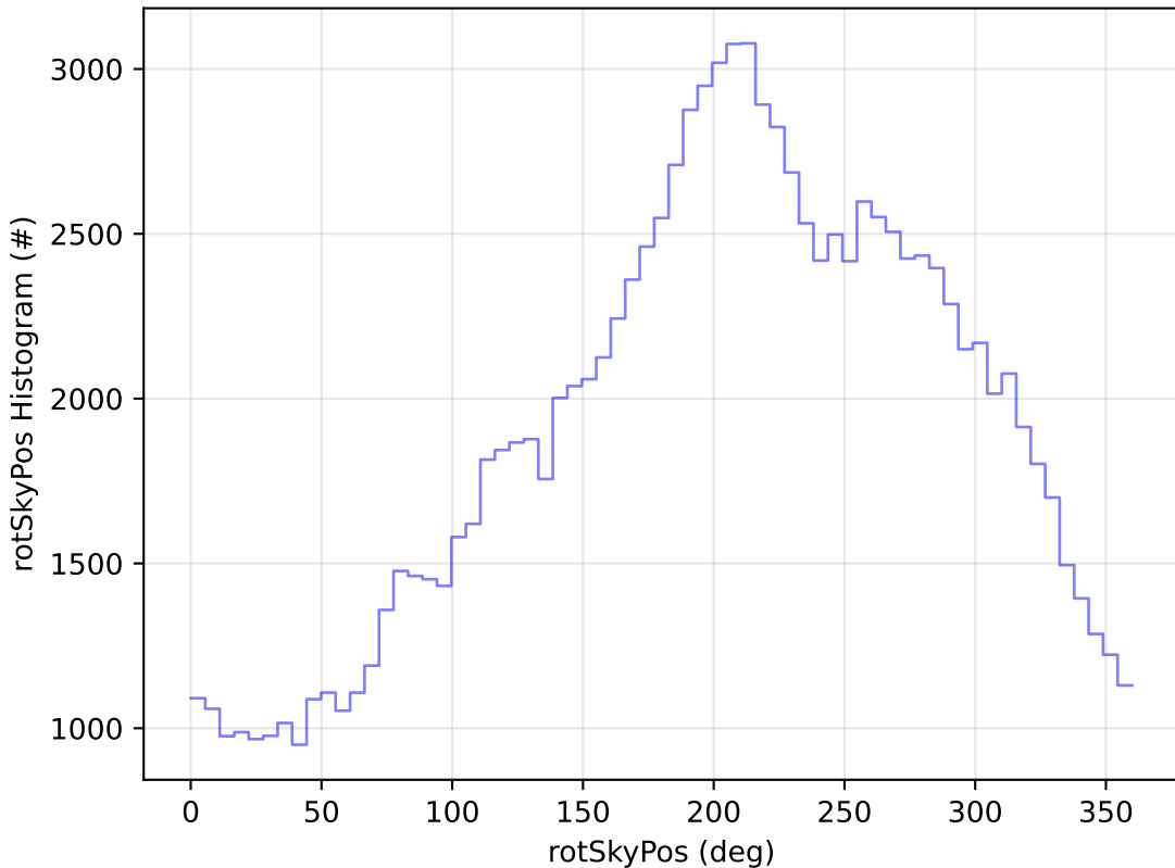
ddf_acor_sf15_lsf40_lsr20_v3.4_10yrs WFD u band: rotSkyPos Histogram
