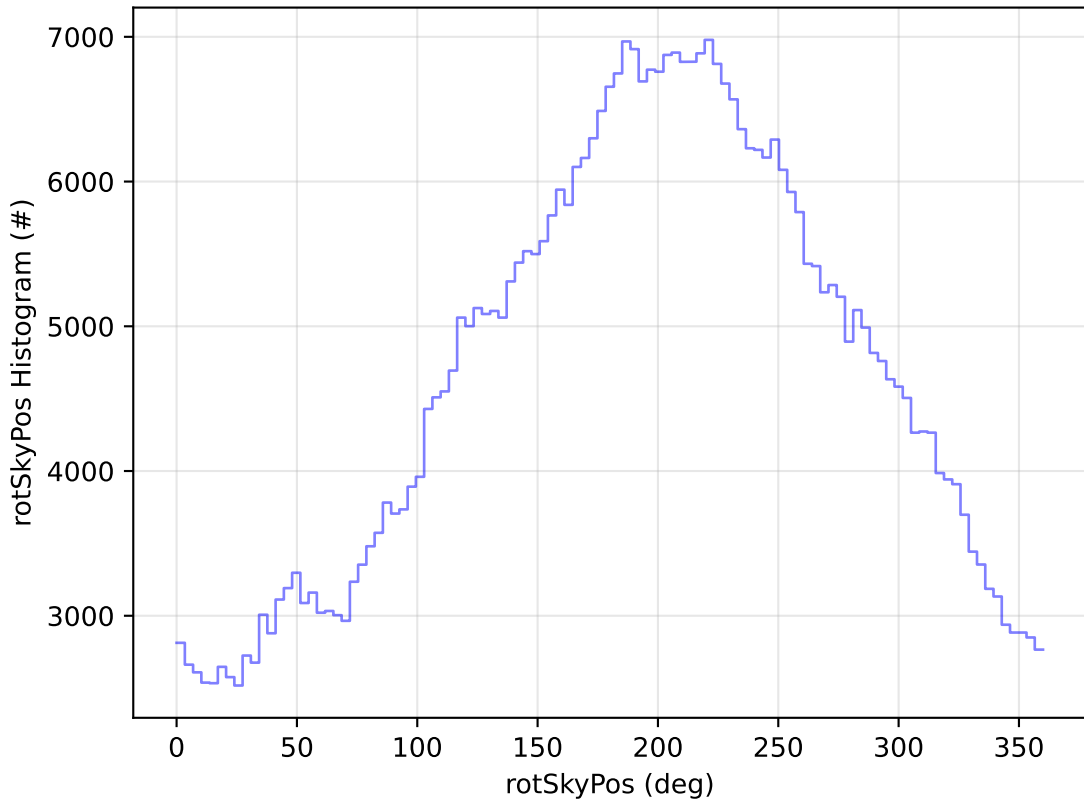
ddf_acor_sf15_lsf40_lsr20_v3.4_10yrs WFD r band: rotSkyPos Histogram
