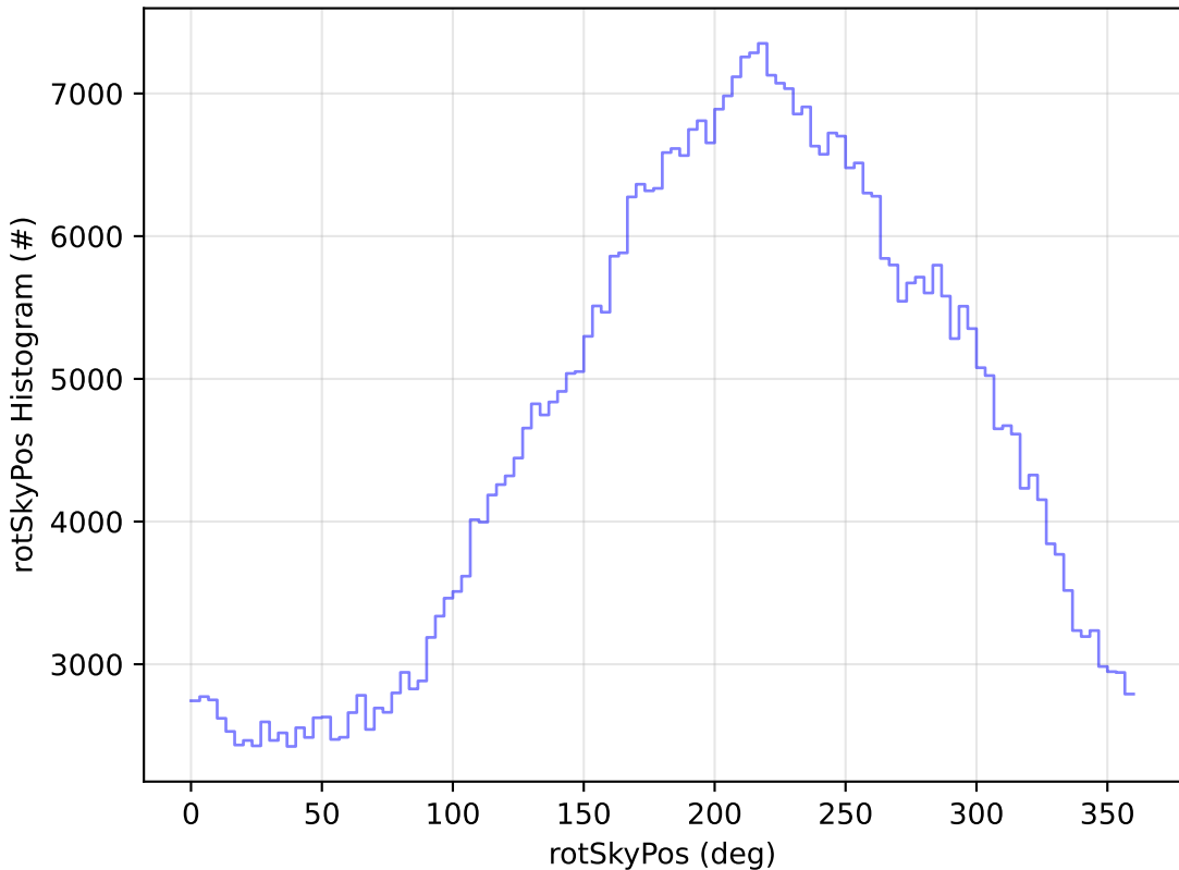
ddf_acor_sf15_lsf40_lsr20_v3.4_10yrs WFD i band: rotSkyPos Histogram
