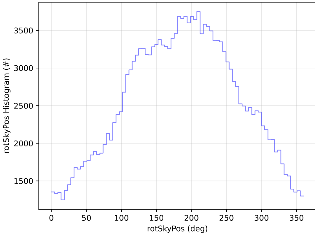
ddf_acor_sf15_lsf40_lsr20_v3.4_10yrs WFD g band: rotSkyPos Histogram
