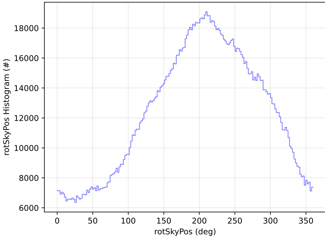
ddf_acor_sf15_lsf40_lsr20_v3.4_10yrs WFD all bands: rotSkyPos Histogram
