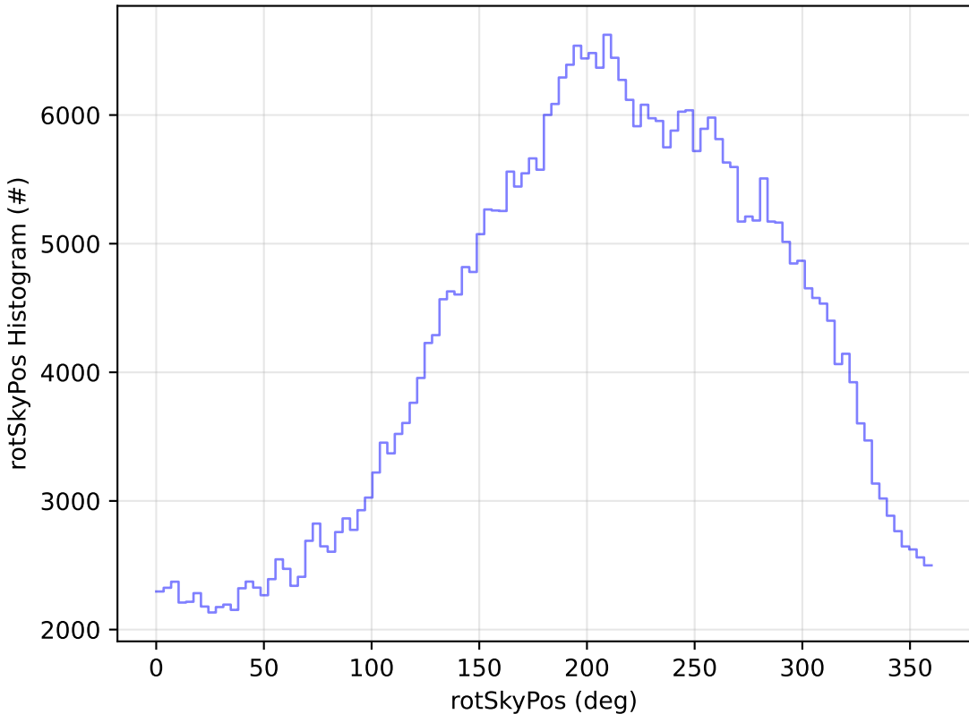
ddf_acor_sf15_lsf40_lsr20_v3.4_10yrs All sky z band: rotSkyPos Histogram
