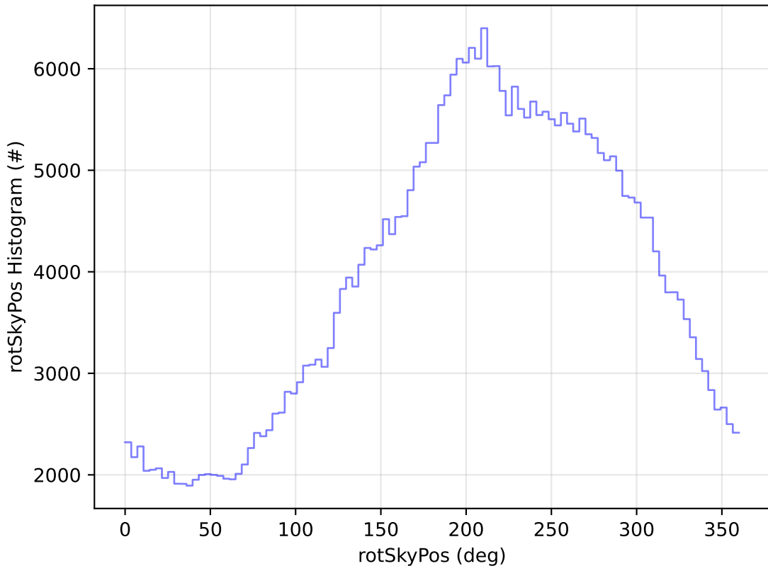
ddf_acor_sf15_lsf40_lsr20_v3.4_10yrs All sky y band: rotSkyPos Histogram
