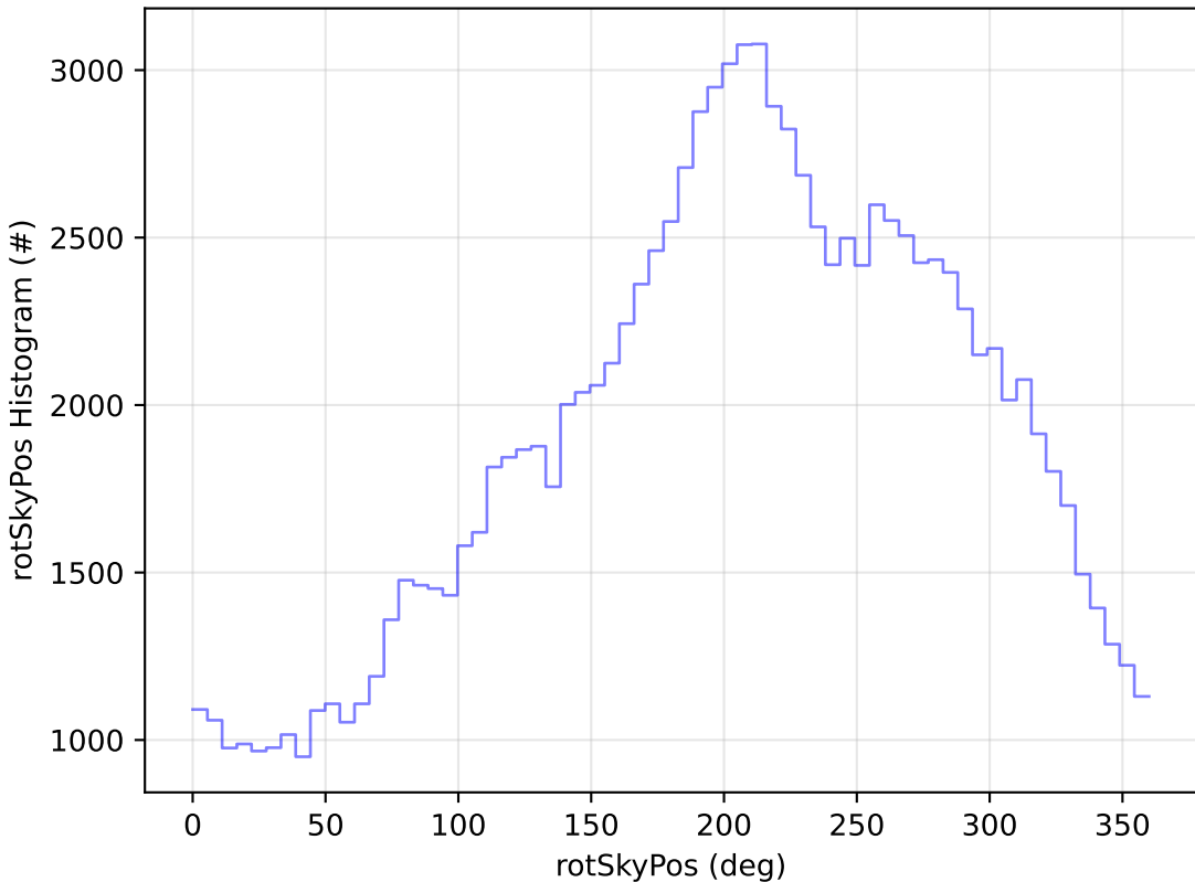
ddf_acor_sf15_lsf40_lsr20_v3.4_10yrs All sky u band: rotSkyPos Histogram
