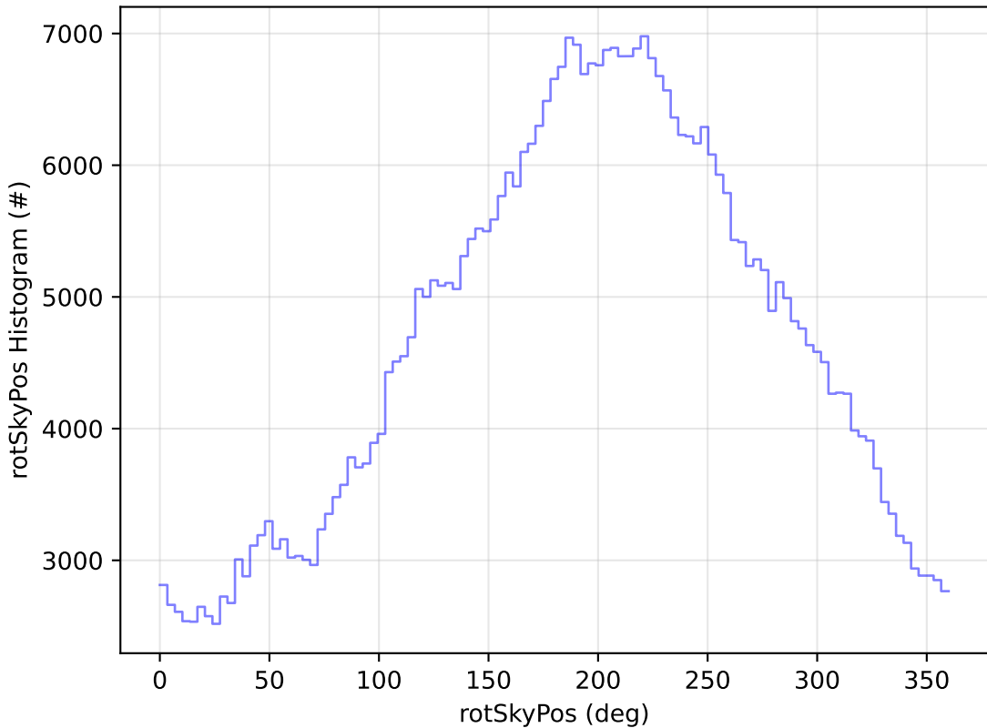
ddf_acor_sf15_ls40_lsr20_v3.4_10yrs All sky r band: rotSkyPos Histogram
